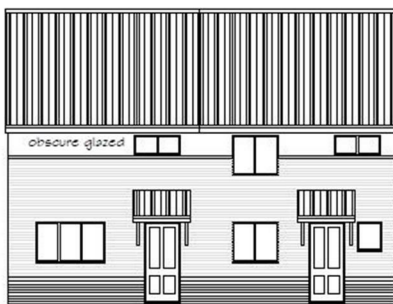
Proposed Front Elevation (north)
